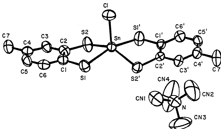
FIGURE 1 ORTEP plot of the complex [(\text{CH}_3)_3\text{N}]^+[(\text{C}_7\text{H}_6\text{S}_2)_2\text{SnCl}]^- (2), with thermal ellipsoids at the 50% probability level.
